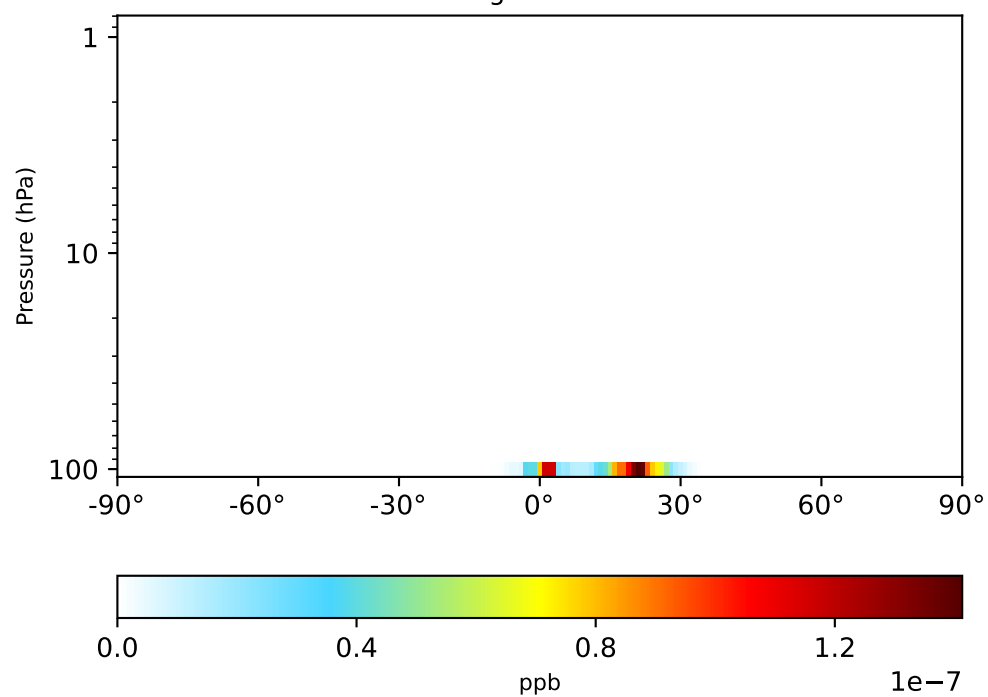
gchp-c24-1Mon-14.7.0-alpha.11 (Dev) 1x1.25 regridded from c24
