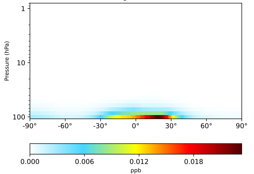
gchp-c24-1Mon-14.7.0-alpha.11 (Dev) 1x1.25 regridded from c24
