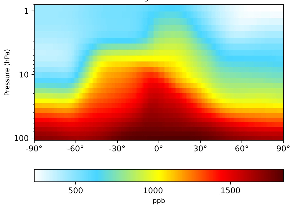
gchp-c24-1Mon-14.7.0-alpha.10 (Ref) 1x1.25 regridded from c24
