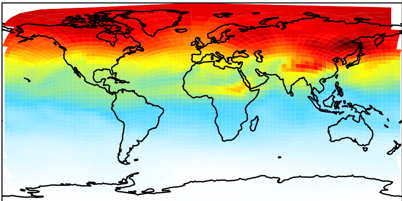
gchp-c24-1Mon-14.7.0-alpha.10 (Ref) c24
