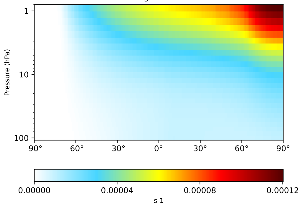
gchp-c24-1Mon-14.7.0-alpha.1 (Ref) 1x1.25 regridded from c24
