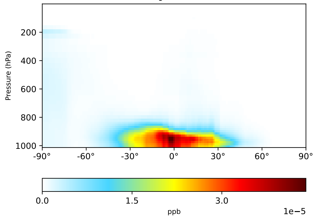
gchp-c24-1Mon-14.7.0-alpha.1 (Ref) 1x1.25 regridded from c24
