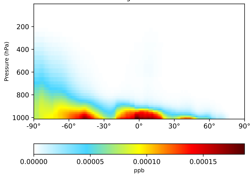
gchp-c24-1Mon-14.7.0-alpha.1 (Ref) 1x1.25 regrided from c24
