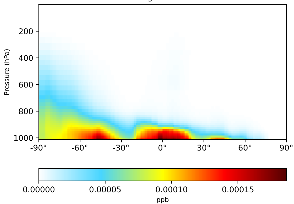
gchp-c24-1Mon-14.7.0-alpha.2 (Dev) 1x1.25 regrided from c24
