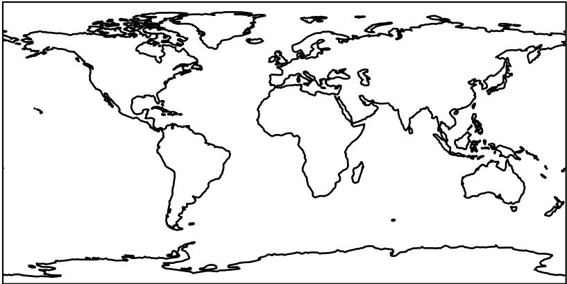
gchp-c24-1Mon-14.7.0-alpha.1 (Ref) c24
