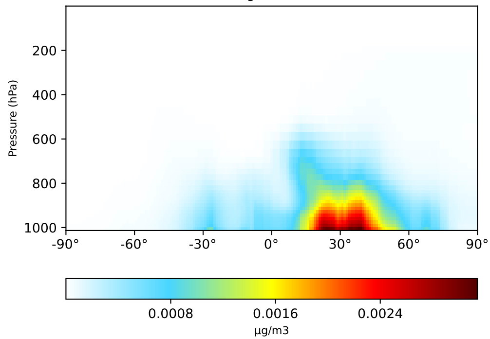
gchp-c24-1Mon-14.7.0-alpha.0 (Ref) 1x1.25 regrided from c24
