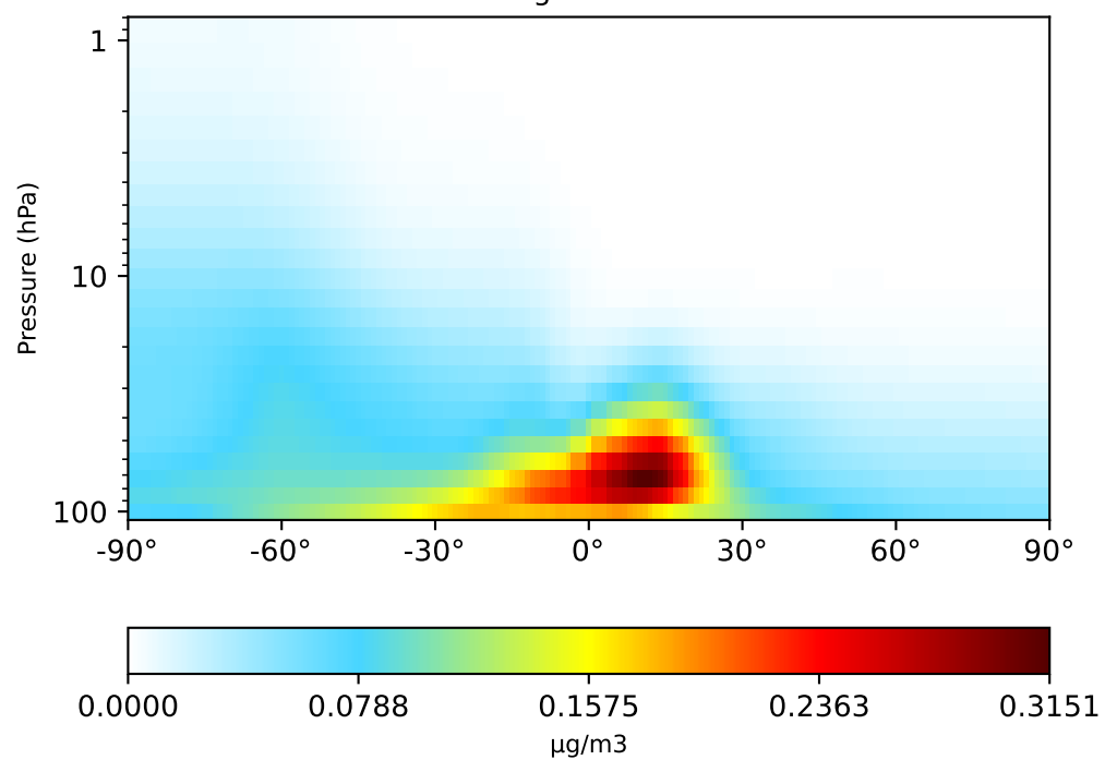
gchp-c24-1Mon-14.7.0-alpha.3 (Dev) 1x1.25 regridded from c24
