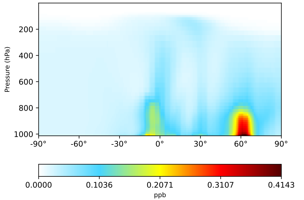
gchp-c24-1Mon-14.7.0-alpha.17 (Dev) 1x1.25 regrided from c24
