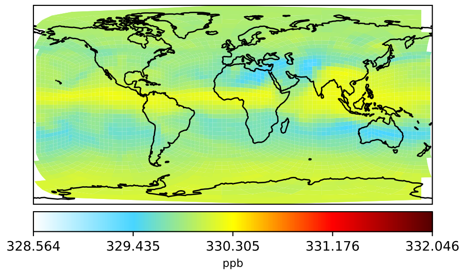
gchp-c24-1Mon-14.6.3 (Ref) c24
