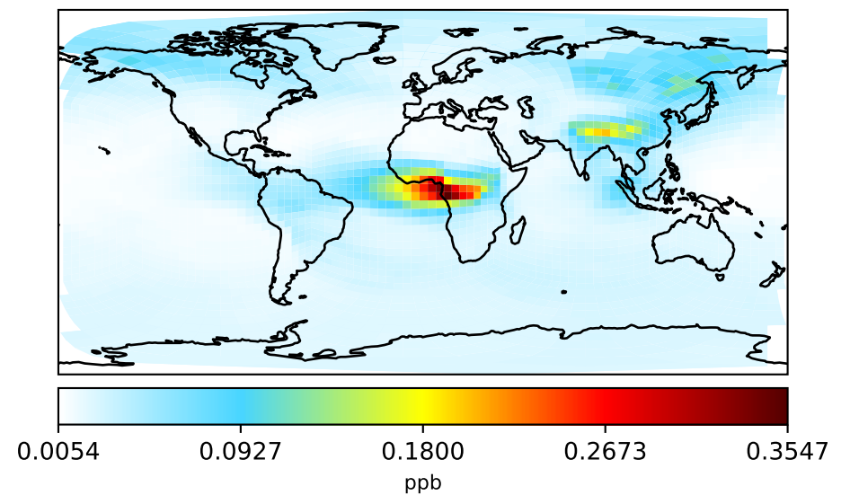
gchp-c24-1Mon-14.7.0-alpha.0 (Dev) c24
