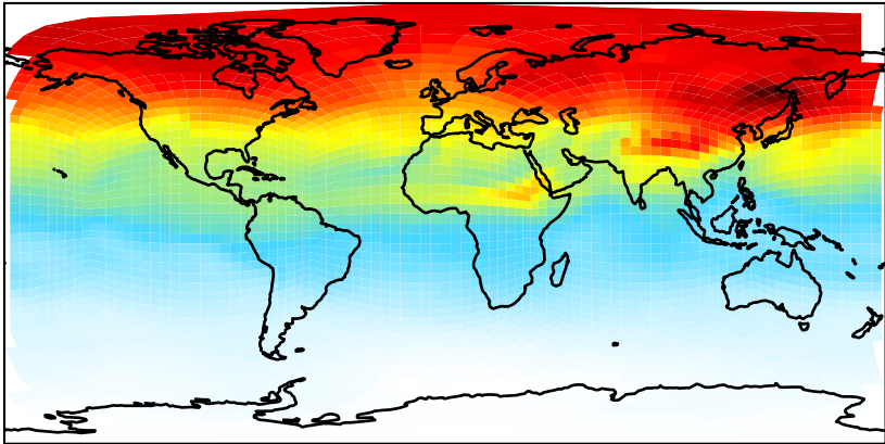
gchp-c24-1Mon-14.6.1 (Ref) c24
