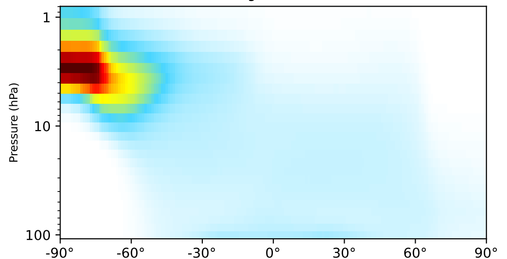
gchp-c24-1Mon-14.6.2 (Dev) 1x1.25 regridded from c24
