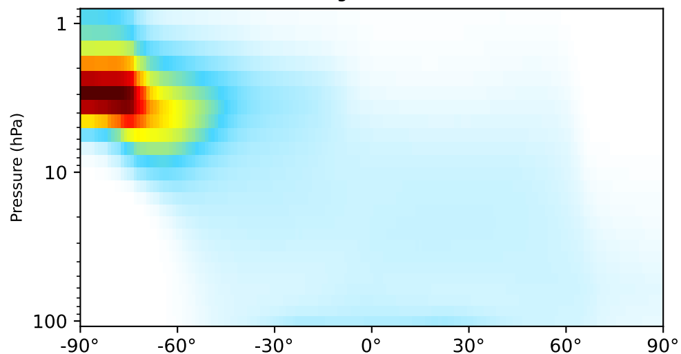
gchp-c24-1Mon-14.6.1 (Ref) 1x1.25 regridded from c24
