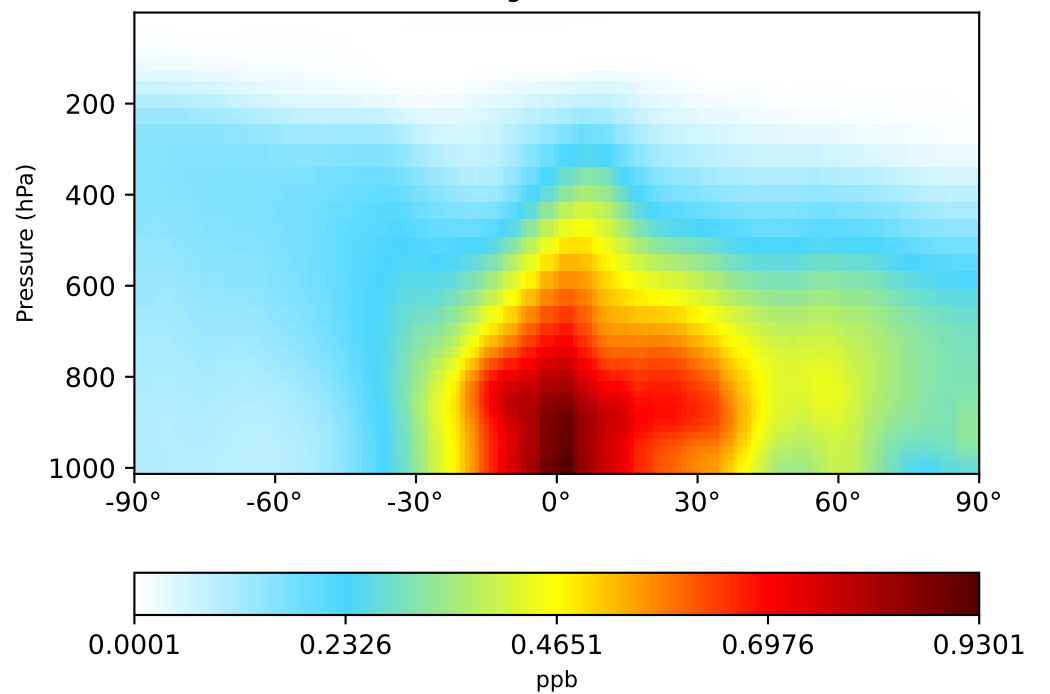
gchp-c24-1Mon-14.6.0-alpha.1 (Dev) 1x1.25 regridded from c24
