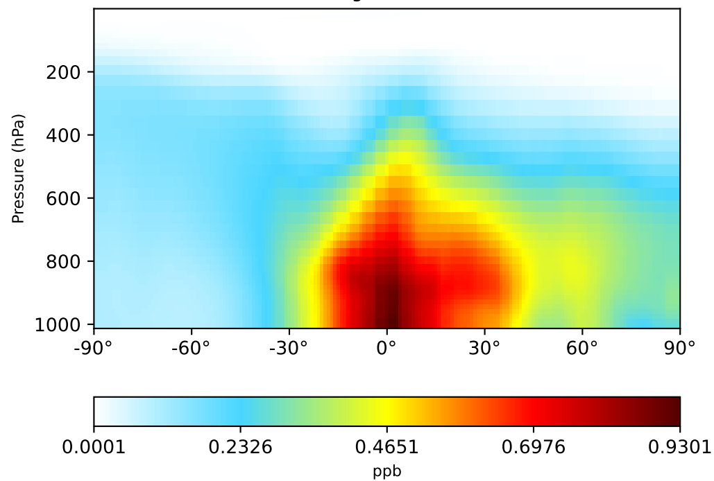
gchp-c24-1Mon-14.5.1 (Ref) 1x1.25 regridded from c24
