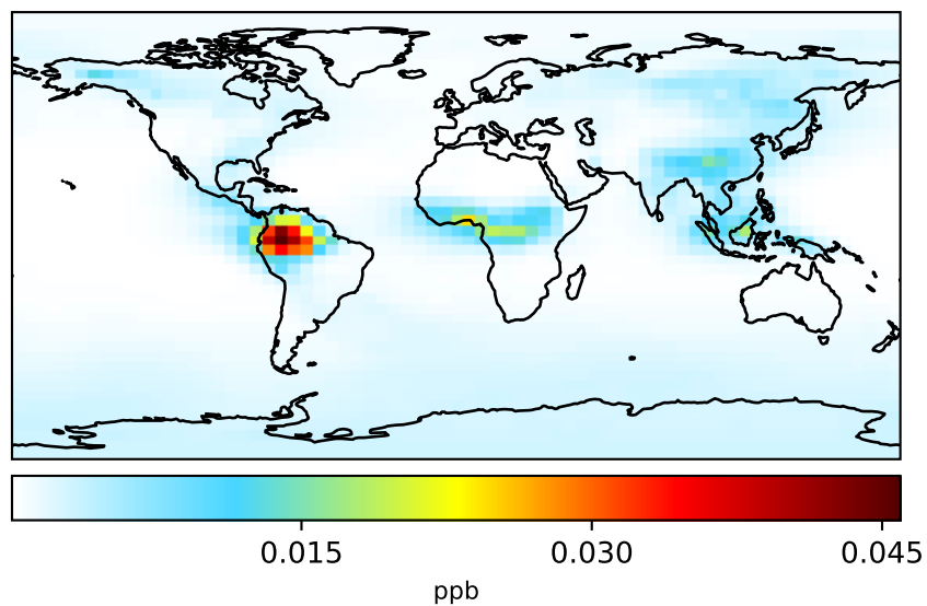
gcc-4x5-1Mon-14.5.0-alpha.4 (Ref) 4.0x5.0
