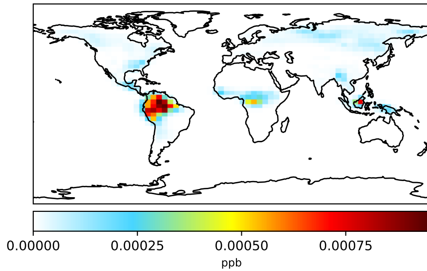
gcc-4x5-1Mon-14.5.0-alpha.4 (Ref) 4.0x5.0
