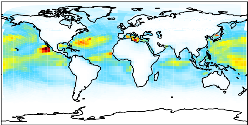
gchp-c24-1Mon-14.5.0-alpha.14 (Ref) c24
