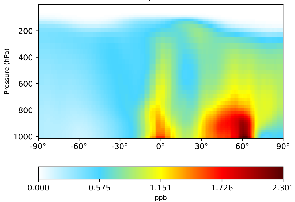
gchp-c24-1Mon-14.5.0-alpha.14 (Dev) 1x1.25 regrided from c24
