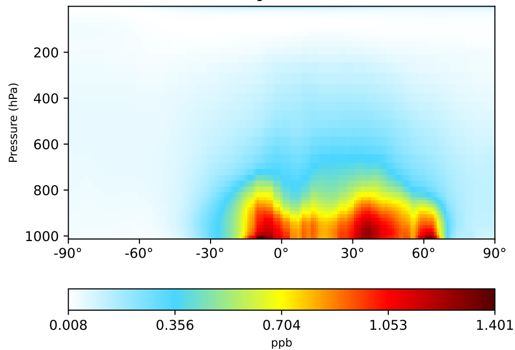
gchp-c24-1Mon-14.5.0-alpha.13 (Ref) 1x1.25 regridded from c24
