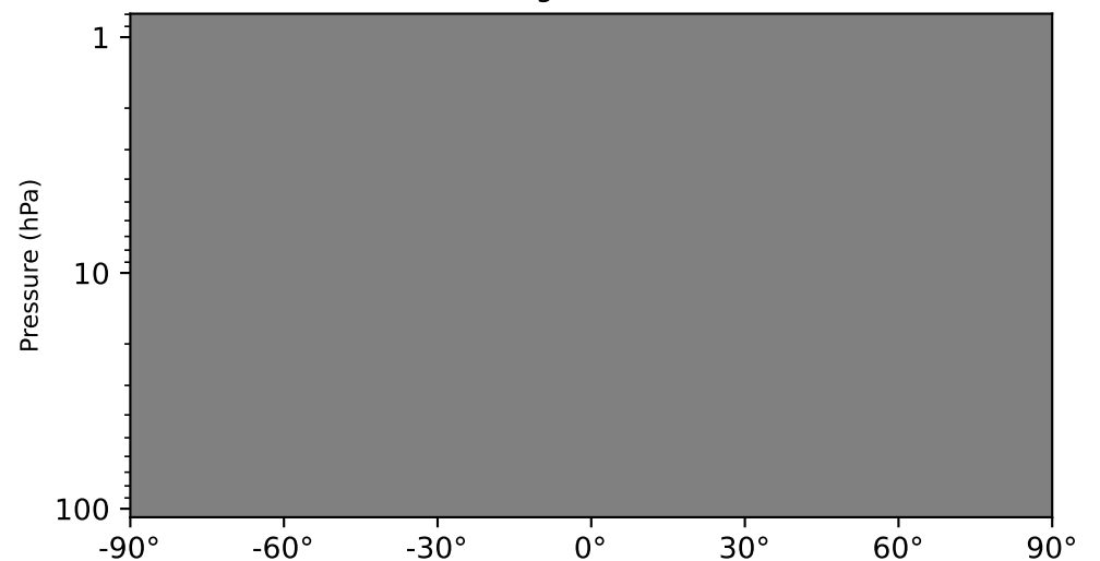
gchp-c24-1Mon-14.5.0-alpha.14 (Dev) 1x1.25 regridded from c24
