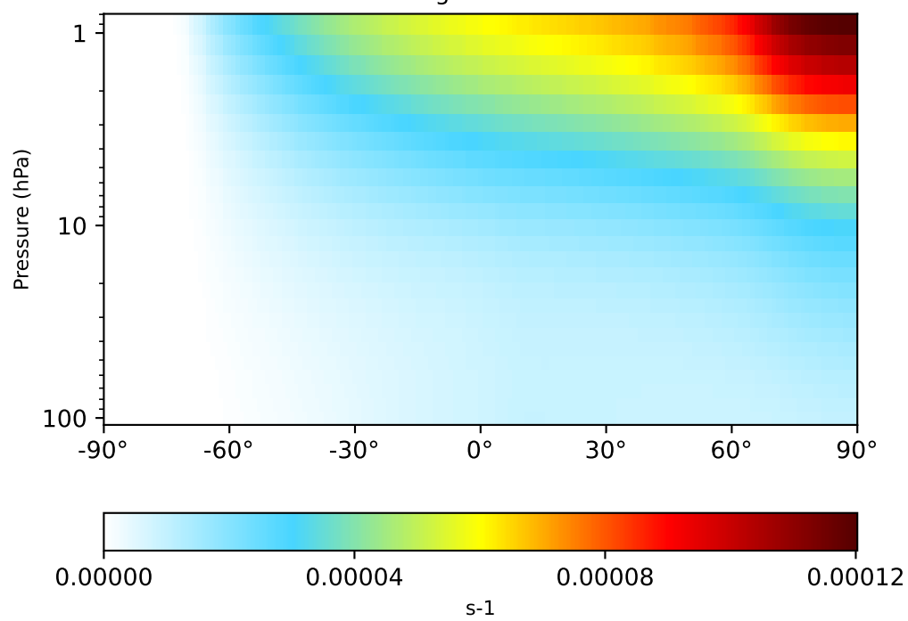
gchp-c24-1Mon-14.5.0-alpha.13 (Ref) 1x1.25 regridded from c24
