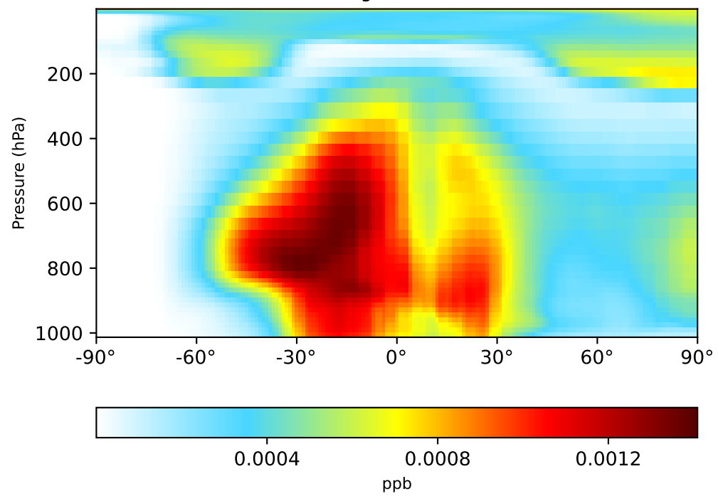
gchp-c24-1Mon-14.5.0-alpha.13 (Ref) 1x1.25 regrided from c24
