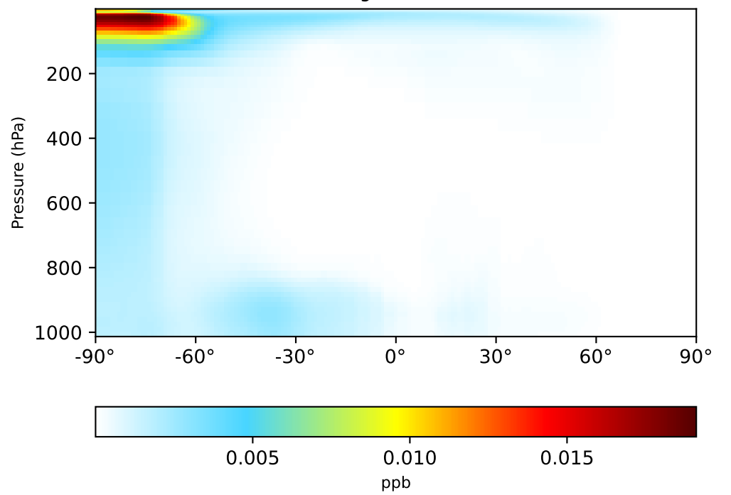
gchp-c24-1Mon-14.5.0-alpha.14 (Dev) 1x1.25 regrided from c24
