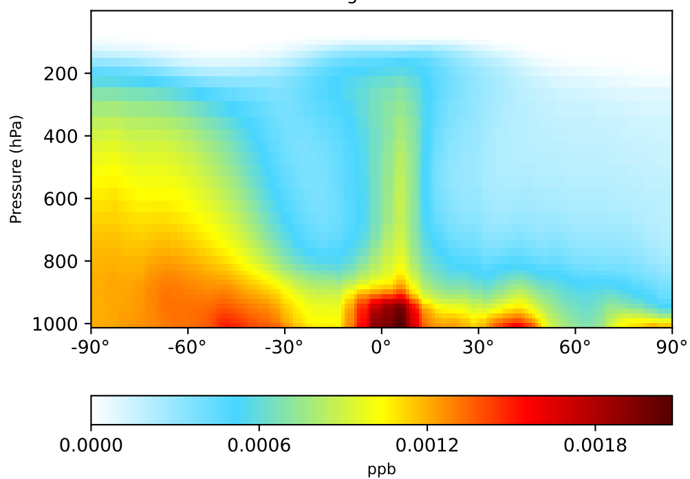
gchp-c24-1Mon-14.5.0-alpha.14 (Dev) 1x1.25 regrided from c24
