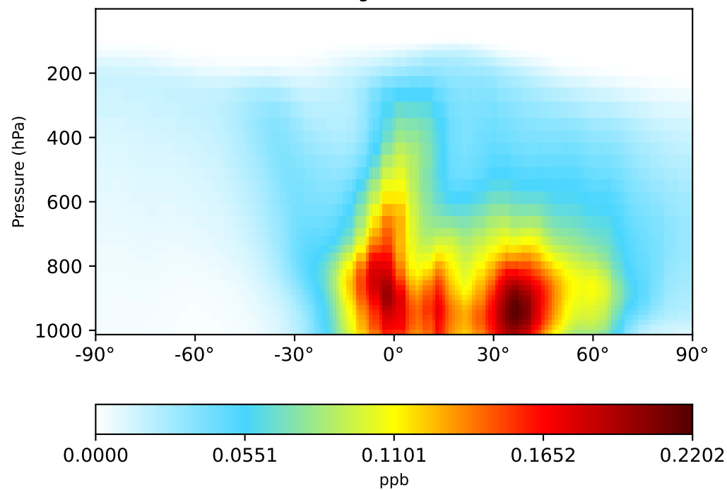
gchp-c24-1Mon-14.5.0-alpha.0 (Ref) 1x1.25 regridded from c24
