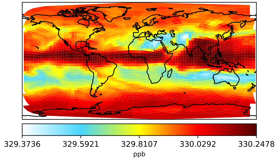
gchp-c24-1Mon-14.5.0-alpha.0 (Ref) c24
