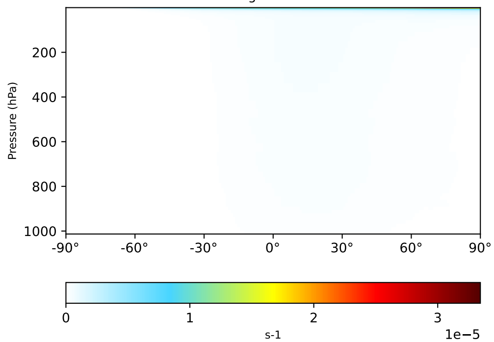
gchp-c24-1Mon-14.5.0-alpha.1 (Dev) 1x1.25 regrided from c24
