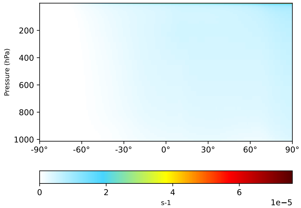
gchp-c24-1Mon-14.5.0-alpha.0 (Ref) 1x1.25 regrided from c24
