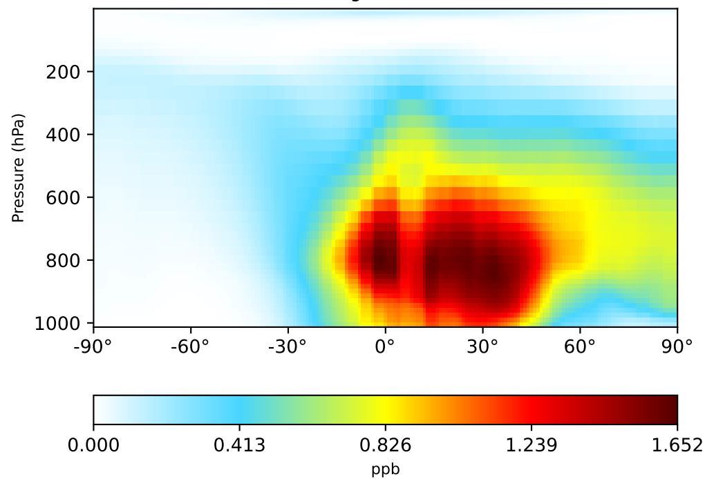
gchp-c24-1Mon-14.4.0-alpha.17 (Ref) 1x1.25 regridded from c24
