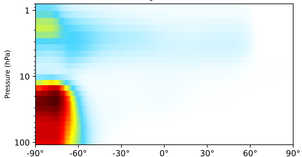
gchp-c24-1Mon-14.4.0-alpha.17 (Ref) 1x1.25 regridded from c24
