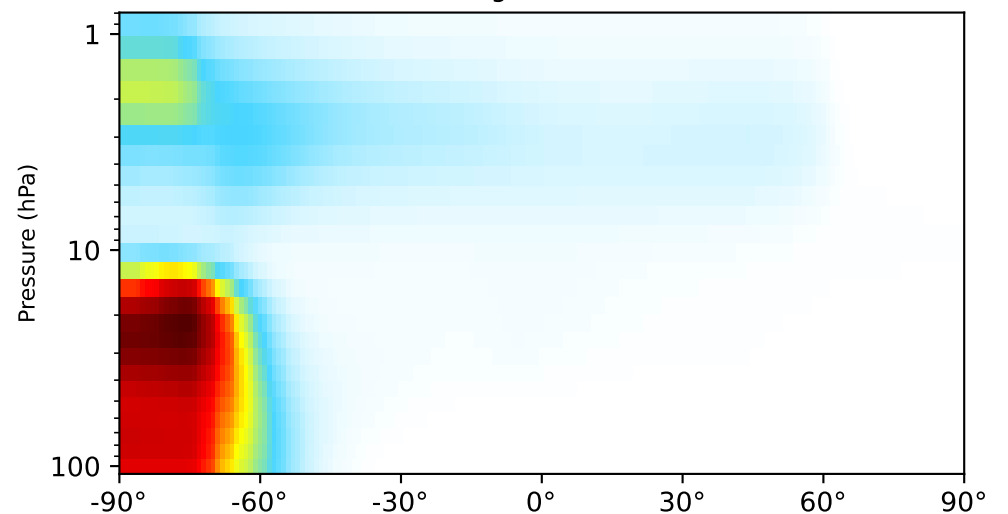
gchp-c24-1Mon-14.4.0 (Dev) 1x1.25 regridded from c24
