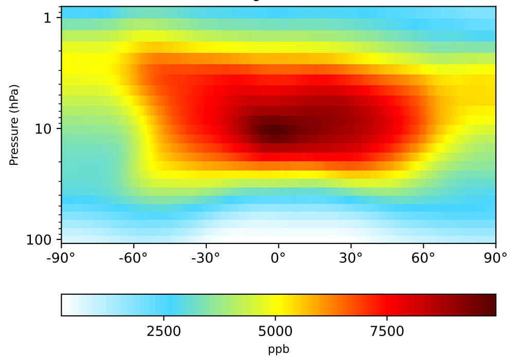
gchp-c24-1Mon-14.3.1 (Dev) 1x1.25 regrided from c24
