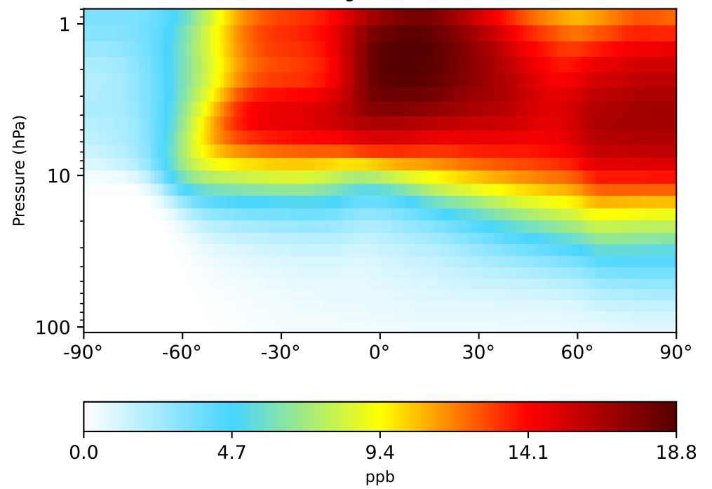
gchp-c24-1Mon-14.3.1 (Dev) 1x1.25 regridded from c24
