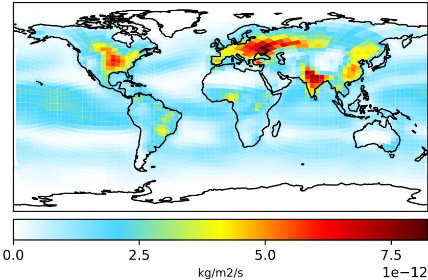
gchp-c24-1Mon-14.3.1 (Dev) c24
