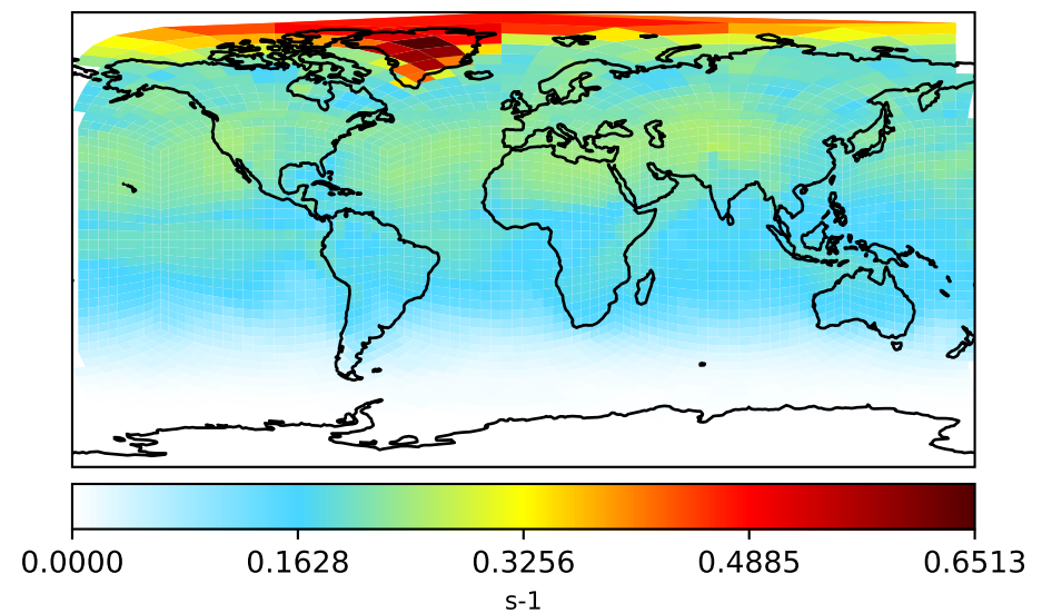
gchp-c24-1Mon-14.3.1 (Dev) c24
