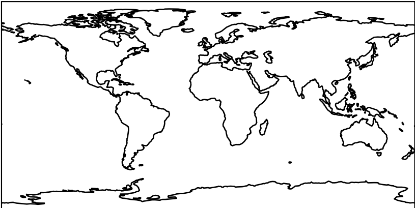
gchp-c24-1Mon-14.3.1 (Dev) c24
