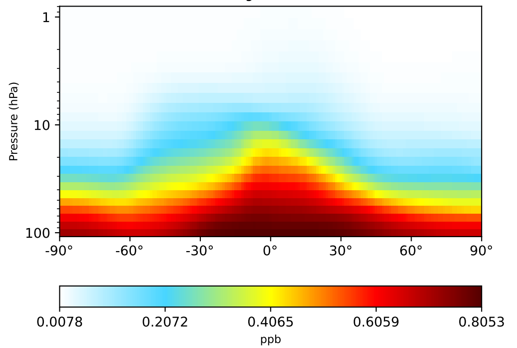
gchp-c24-1Mon-14.3.1 (Dev) 1x1.25 regrided from c24
