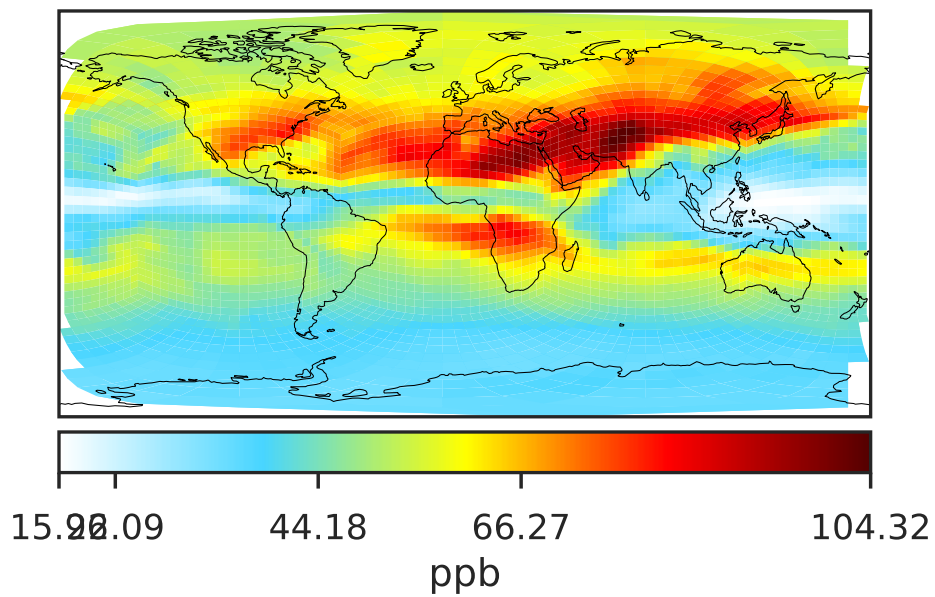
gchp-c24-1Mon-14.2.0 (Ref) c24
