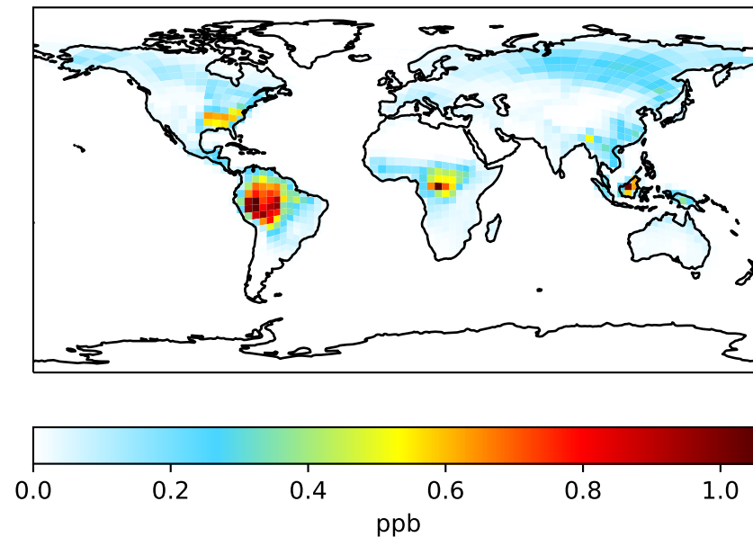
gchp-c24-1Mon-14.2.0-alpha.9 (Dev) c24
