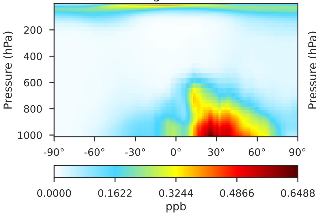
gchp-c24-1Mon-14.1.1 (Ref) 1x1.25 regridded from c24
