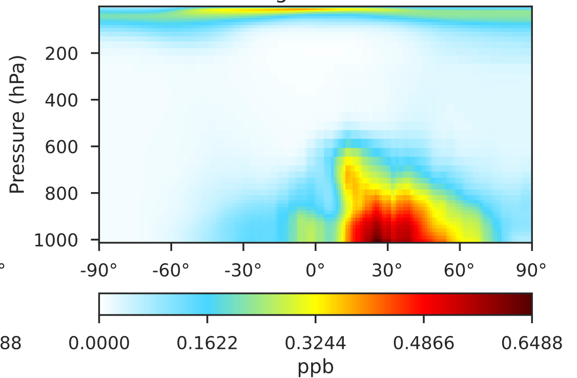
gchp-c24-1Mon-14.2.0-alpha.20 (Dev) 1x1.25 regridded from c24
