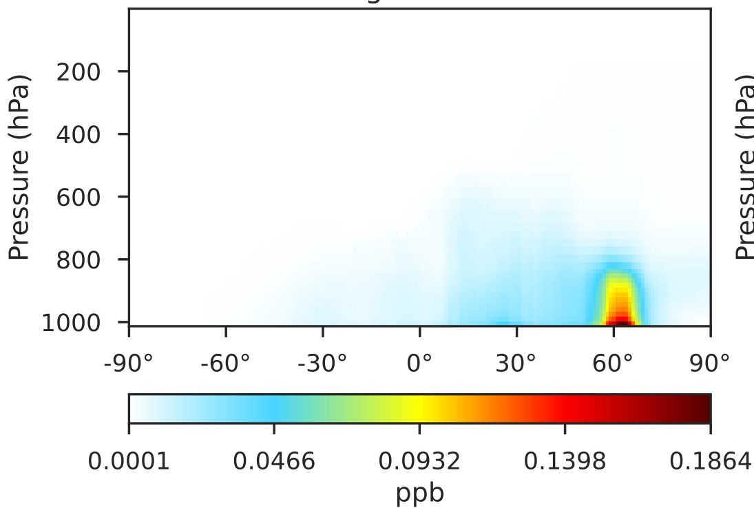
gchp-c24-1Mon-14.1.1 (Ref) 1x1.25 regrided from c24
