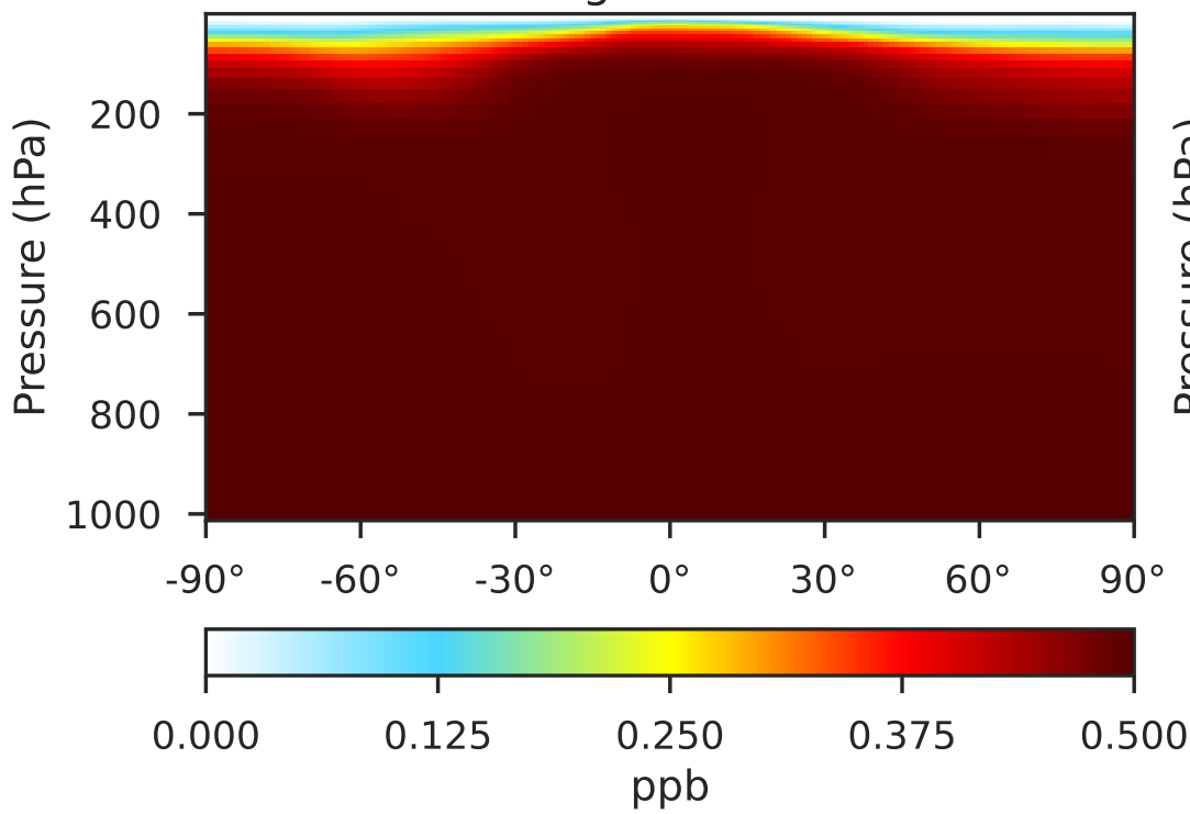
gchp-c24-1Mon-14.1.1 (Ref) 1x1.25 regridded from c24
