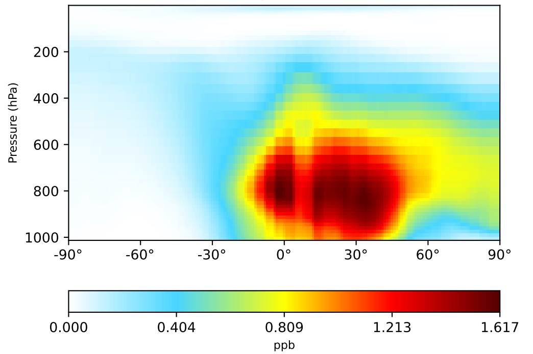
gchp-c24-1Mon-14.7.0-alpha.9 (Dev) 1x1.25 regrided from c24
