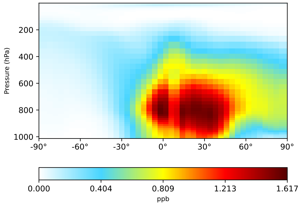
gcc-4x5-1Mon-14.7.0-alpha.9 (Ref) 4.0x5.0
