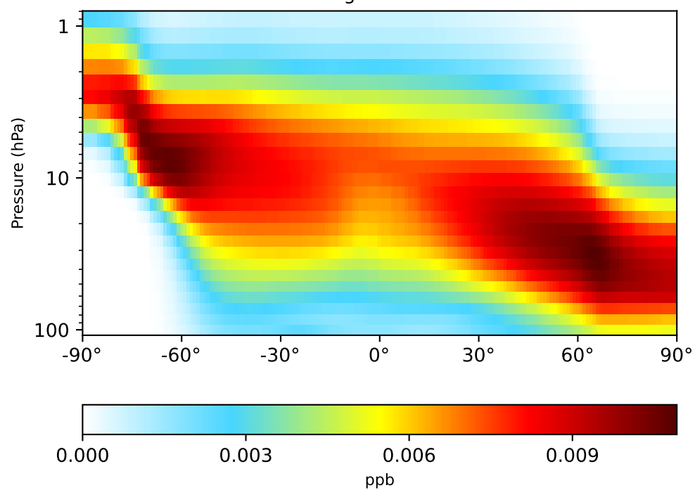
gchp-c24-1Mon-14.7.0-alpha.9 (Dev) 1x1.25 regrided from c24
