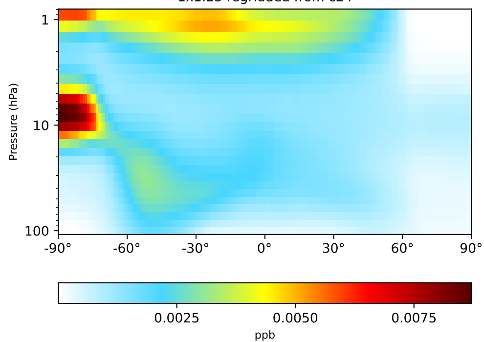
gchp-c24-1Mon-14.7.0-alpha.9 (Dev) 1x1.25 regridged from c24
