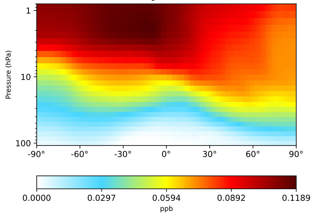
gchp-c24-1Mon-14.7.0-alpha.8 (Dev) 1x1.25 regrided from c24
