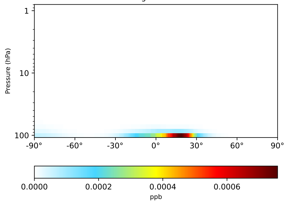
gchp-c24-1Mon-14.7.0-alpha.8 (Dev) 1x1.25 regrided from c24
