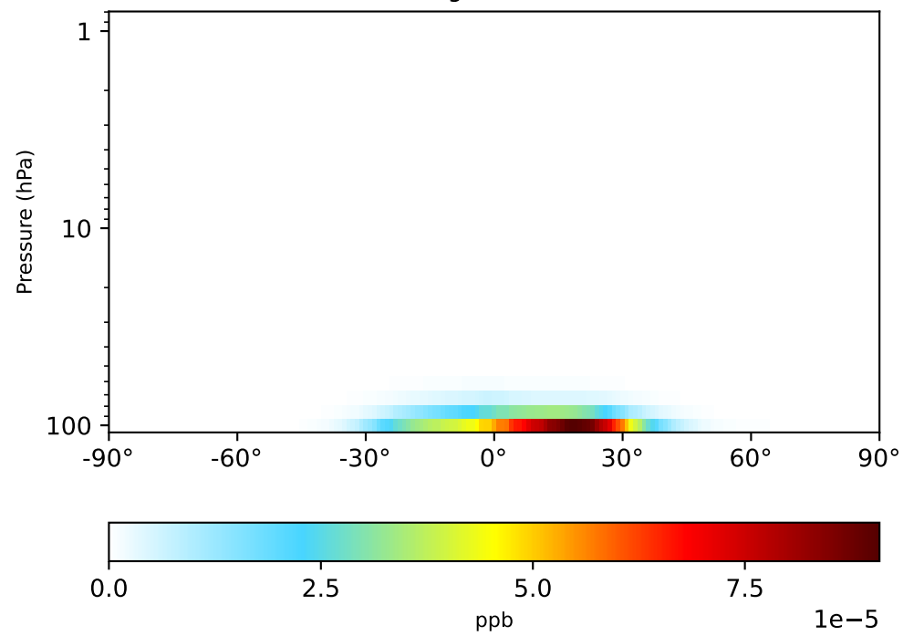
gchp-c24-1Mon-14.7.0-alpha.8 (Dev) 1x1.25 regrided from c24
