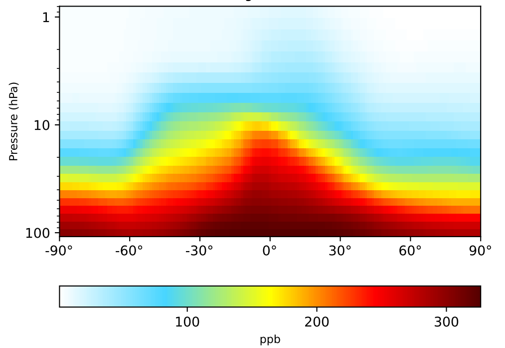
gchp-c24-1Mon-14.7.0-alpha.7 (Dev) 1x1.25 regrided from c24
