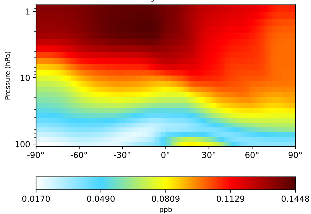
gchp-c24-1Mon-14.7.0-alpha.7 (Dev) 1x1.25 regridded from c24
