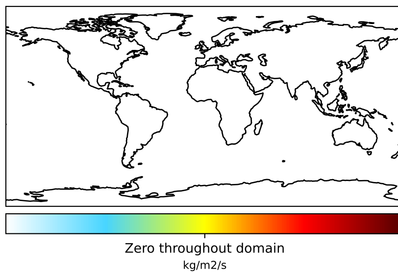
gchp-c24-1Mon-14.7.0-alpha.7 (Dev) c24
