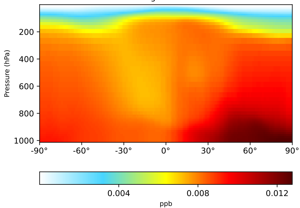
gchp-c24-1Mon-14.7.0-alpha.7 (Dev) 1x1.25 regrided from c24
