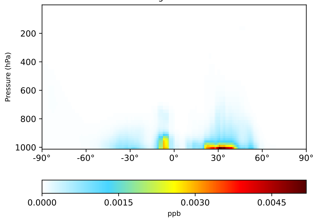
gchp-c24-1Mon-14.7.0-alpha.7 (Dev) 1x1.25 regridded from c24
