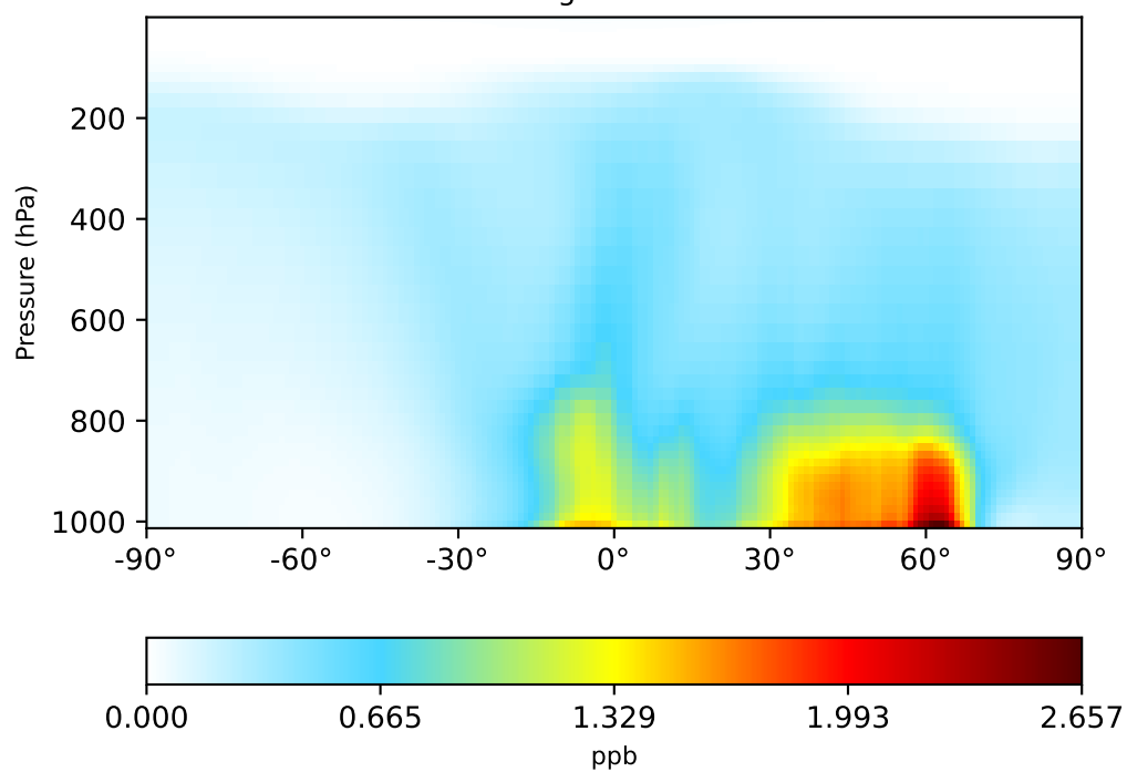
gchp-c24-1Mon-14.7.0-alpha.6 (Dev) 1x1.25 regridded from c24
