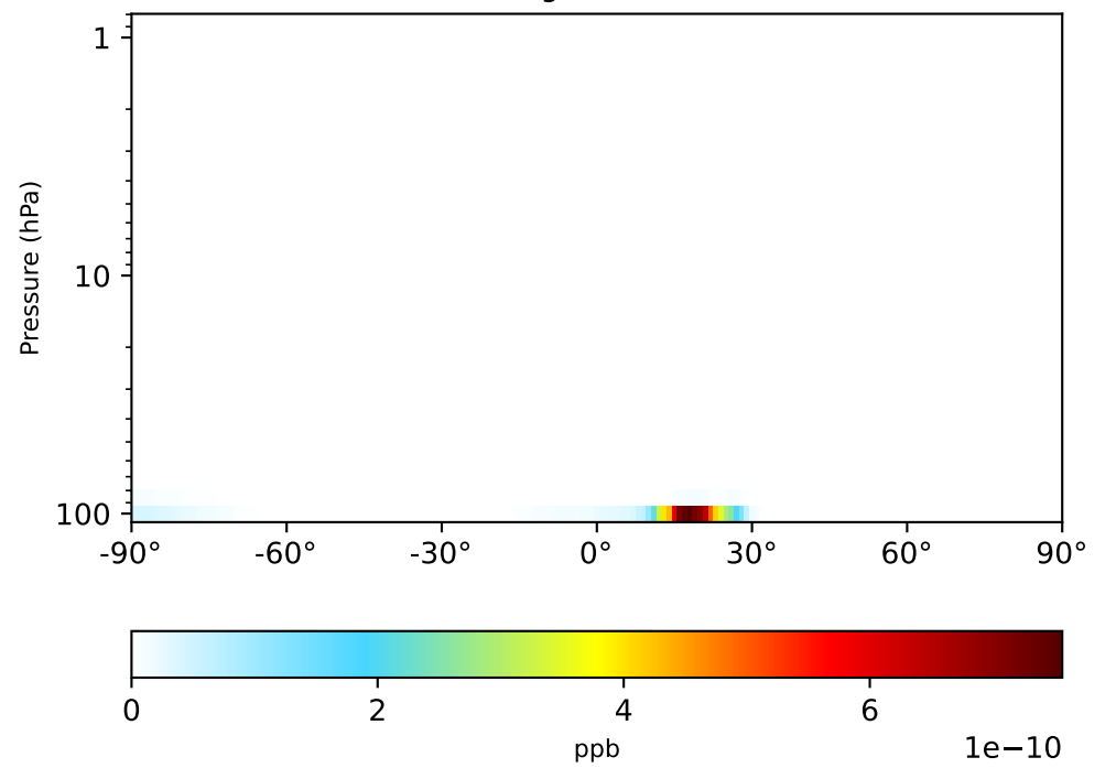
gchp-c24-1Mon-14.7.0-alpha.6 (Dev) 1x1.25 regrided from c24
