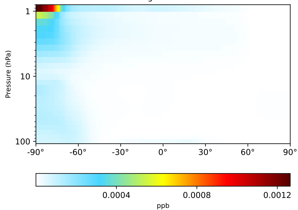
gchp-c24-1Mon-14.7.0-alpha.6 (Dev) 1x1.25 regridded from c24
