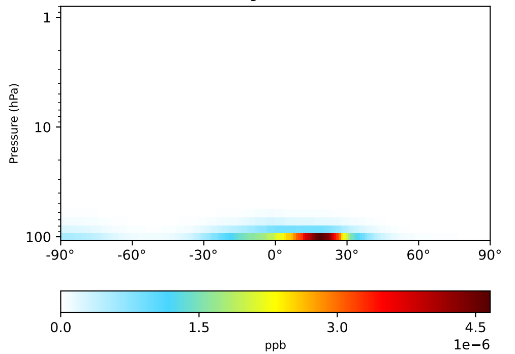
gchp-c24-1Mon-14.7.0-alpha.5 (Dev) 1x1.25 regrided from c24
