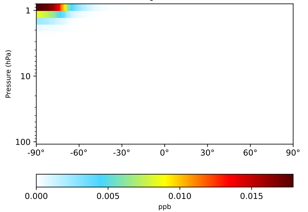
gchp-c24-1Mon-14.7.0-alpha.4 (Dev) 1x1.25 regrided from c24
