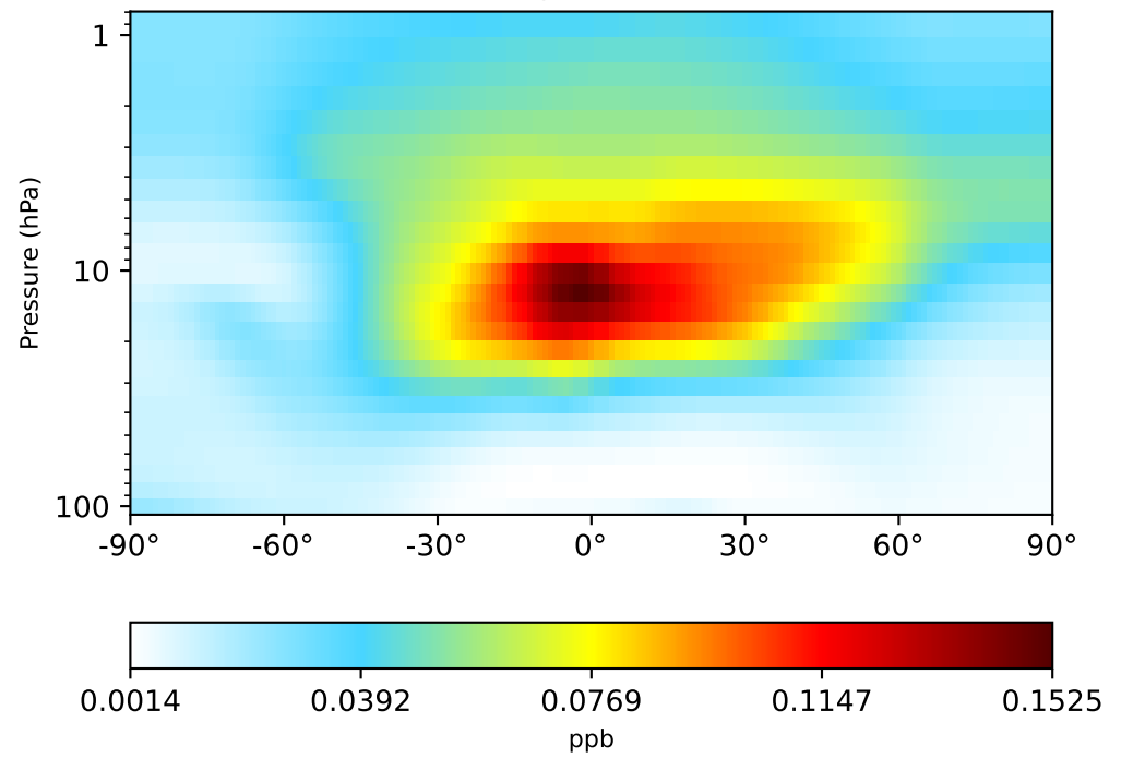
gchp-c24-1Mon-14.7.0-alpha.4 (Dev) 1x1.25 regrided from c24
