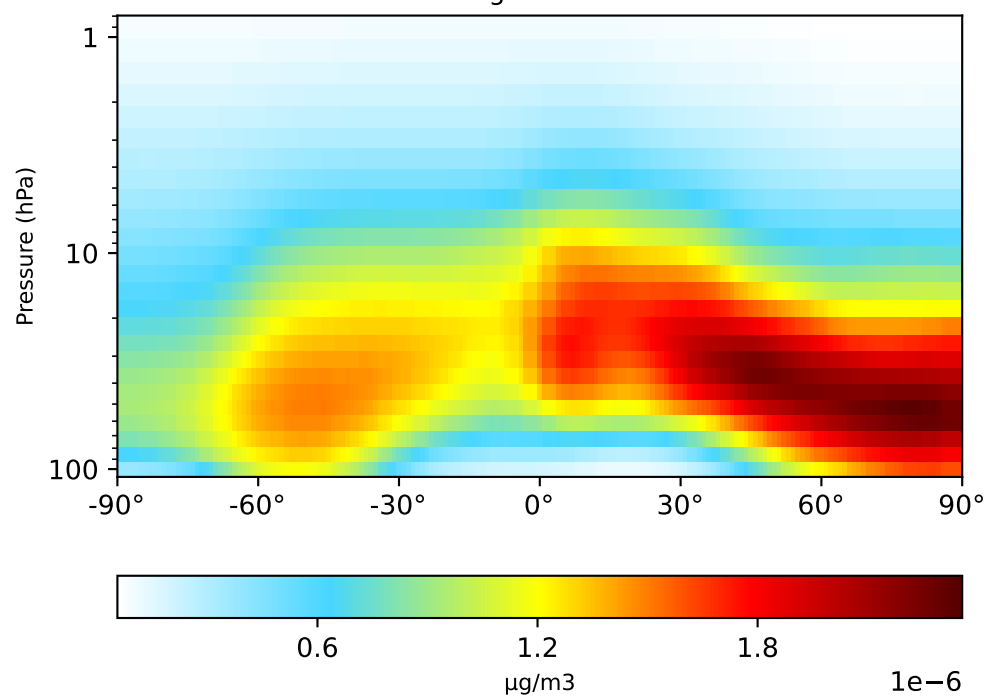
gchp-c24-1Mon-14.7.0-alpha.4 (Dev) 1x1.25 regrided from c24
