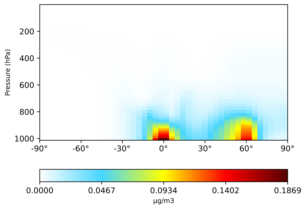
gcc-4x5-1Mon-14.7.0-alpha.4 (Ref) 4.0x5.0
