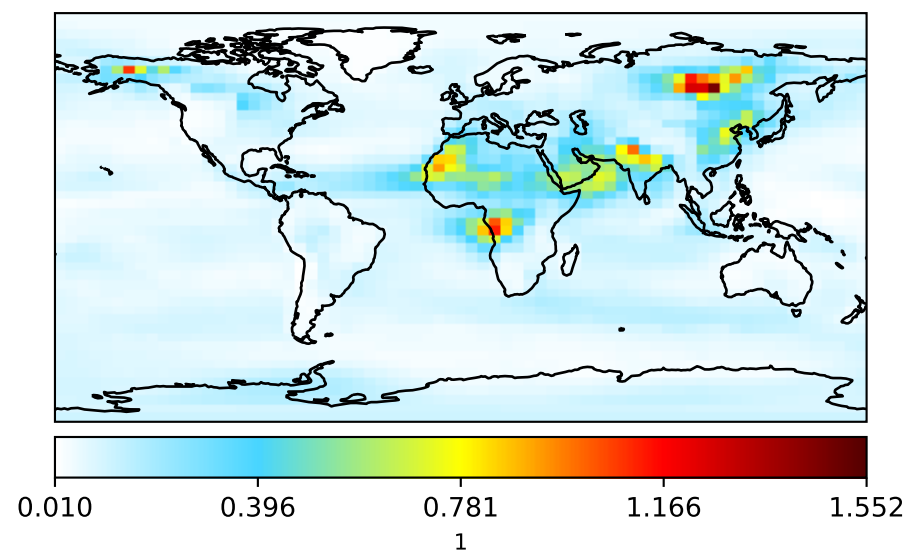
gcc-4x5-1Mon-14.7.0-alpha.5 (Dev) 4.0x5.0
