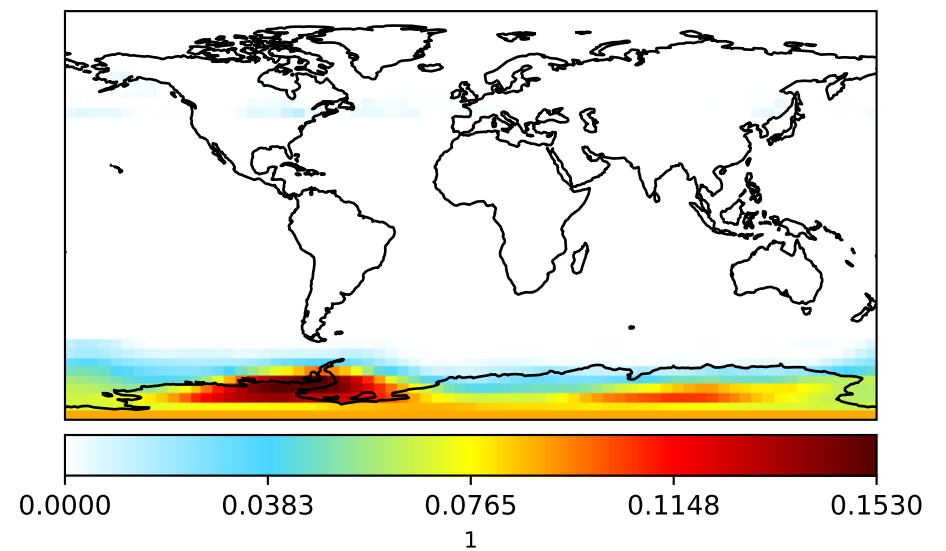
gcc-4x5-1Mon-14.7.0-alpha.5 (Dev) 4.0x5.0
