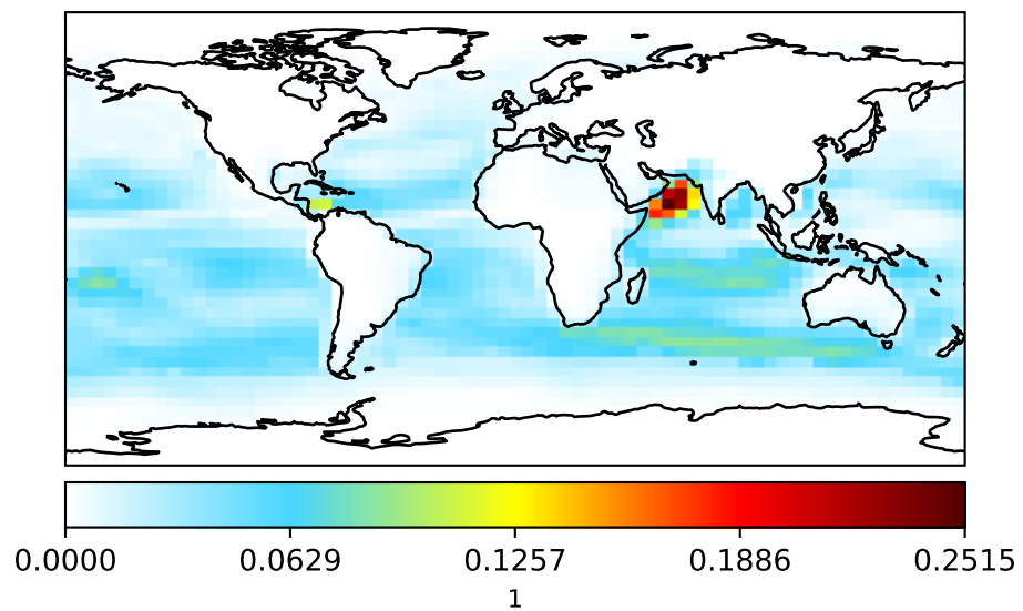
gcc-4x5-1Mon-14.7.0-alpha.4 (Ref) 4.0x5.0
