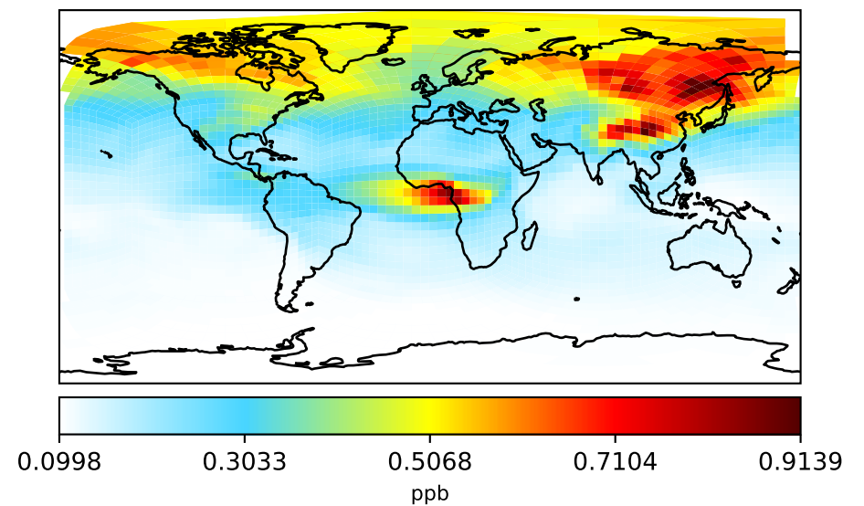
gchp-c24-1Mon-14.7.0-alpha.3 (Dev) c24
