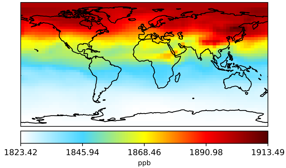
gcc-4x5-1Mon-14.7.0-alpha.3 (Ref) 4.0x5.0
