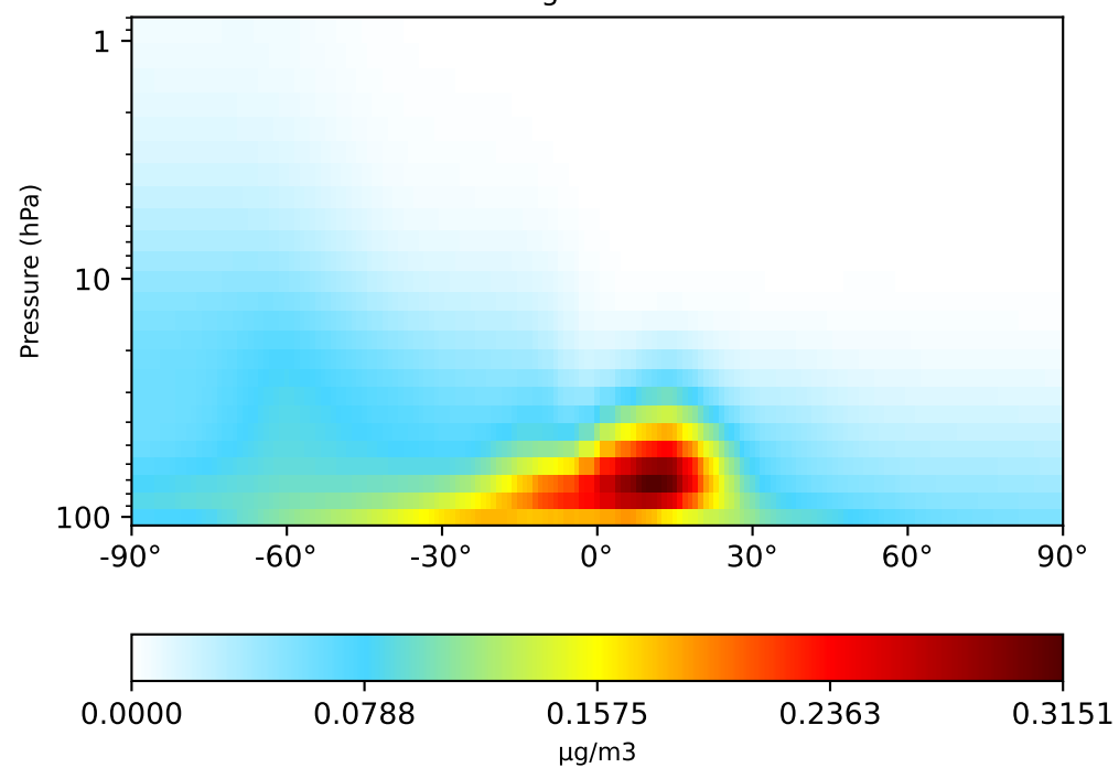
gchp-c24-1Mon-14.7.0-alpha.3 (Dev) 1x1.25 regrided from c24
