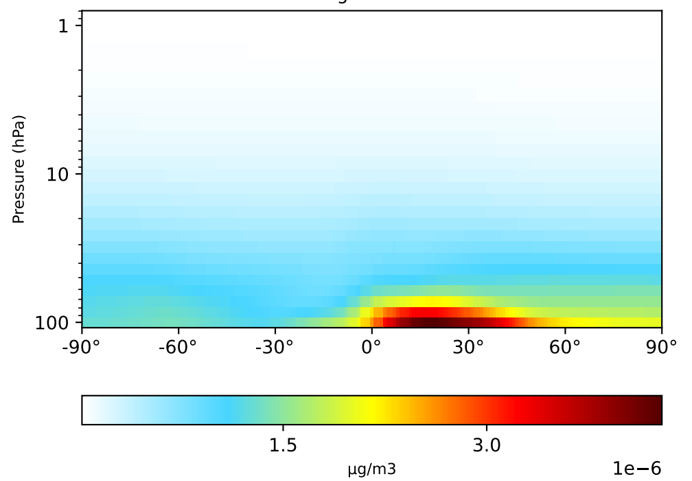
gchp-c24-1Mon-14.7.0-alpha.3 (Dev) 1x1.25 regrided from c24
