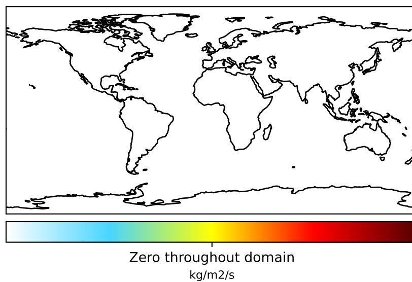
gchp-c24-1Mon-14.7.0-alpha.2 (Dev) c24
