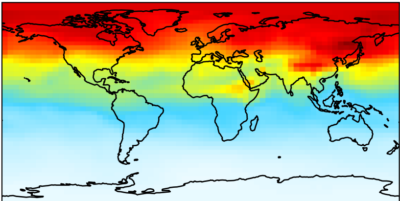
gcc-4x5-1Mon-14.7.0-alpha.18 (Ref) 4.0x5.0
