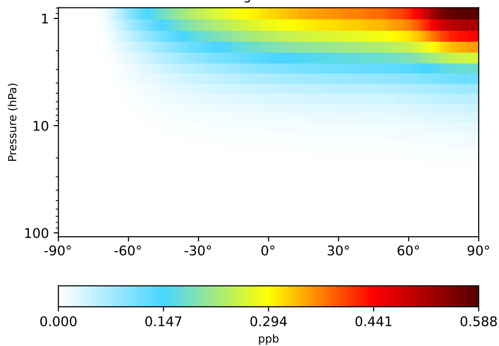
gchp-c24-1Mon-14.7.0-alpha.17 (Dev) 1x1.25 regridded from c24
