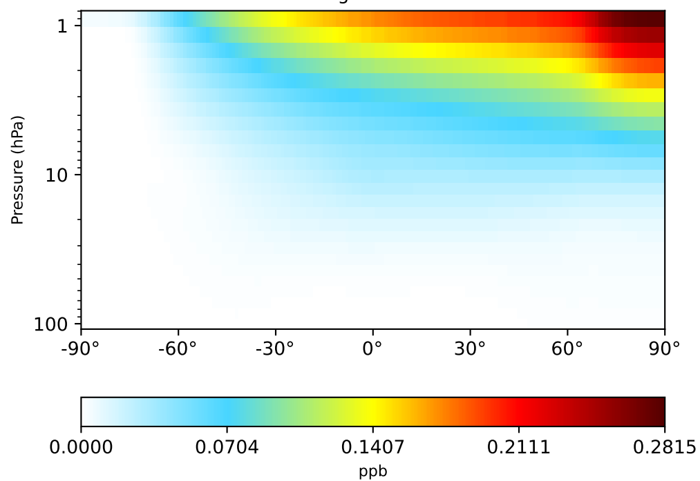
gchp-c24-1Mon-14.7.0-alpha.17 (Dev) 1x1.25 regridded from c24
